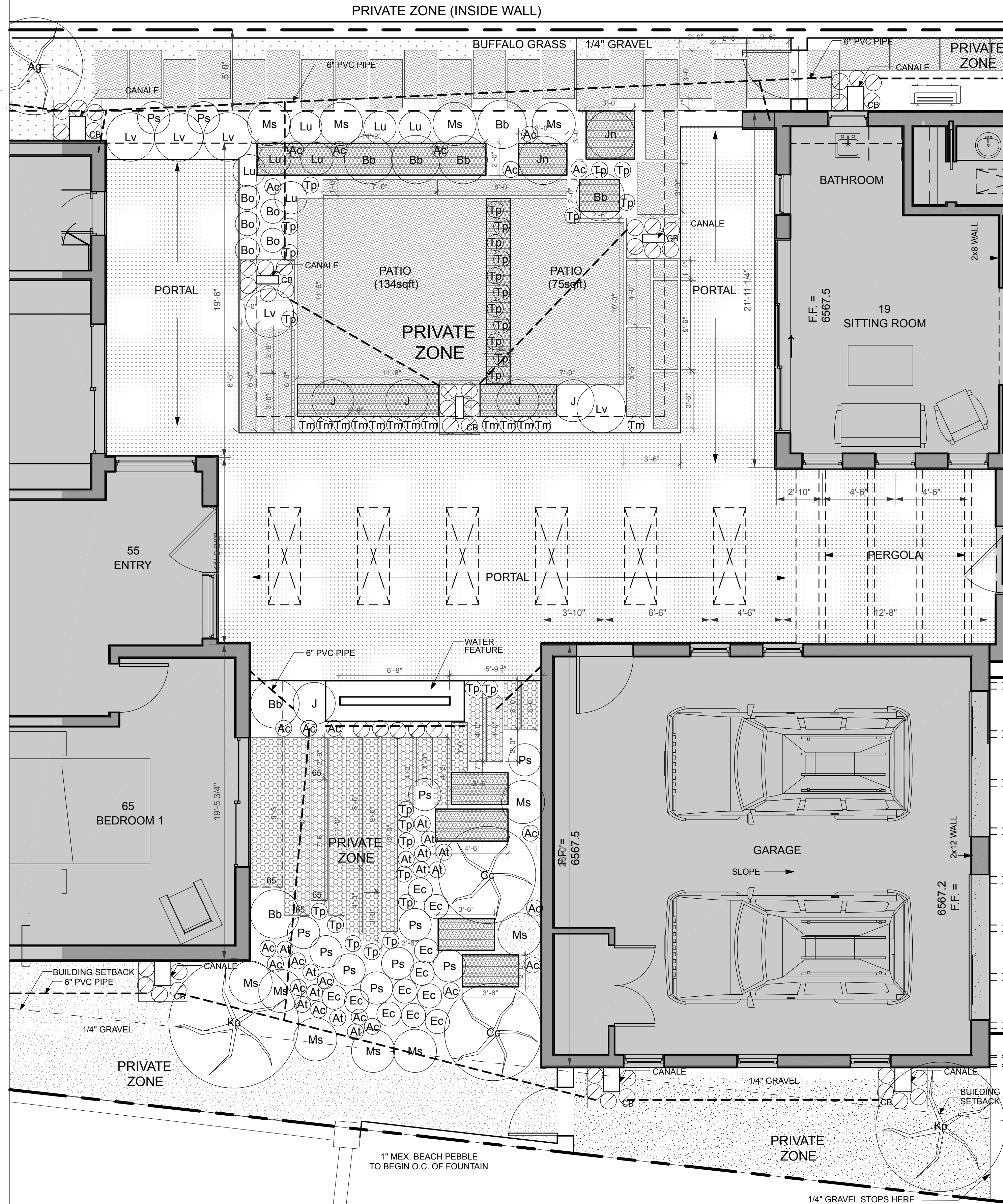
1 LANDSCAPE PLAN - COURTYARD 1/4" = 1'
